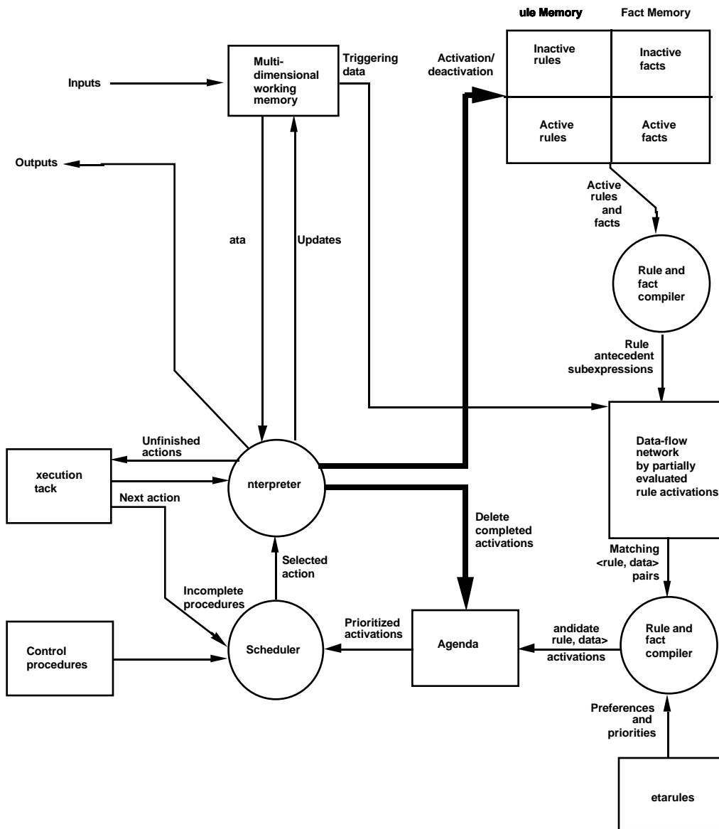
Figure 23: Sophisticated Rule-Based System
