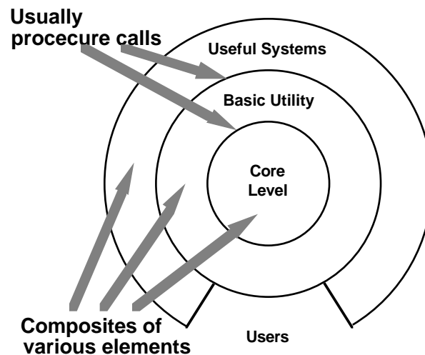
Figure 3: Layered Systems
