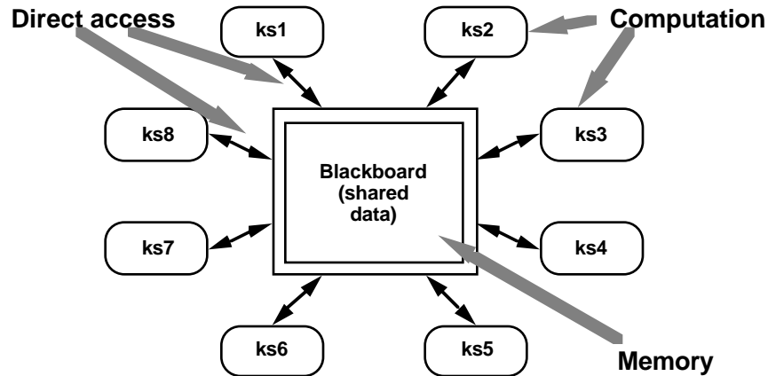
Figure 4: The Blackboard
